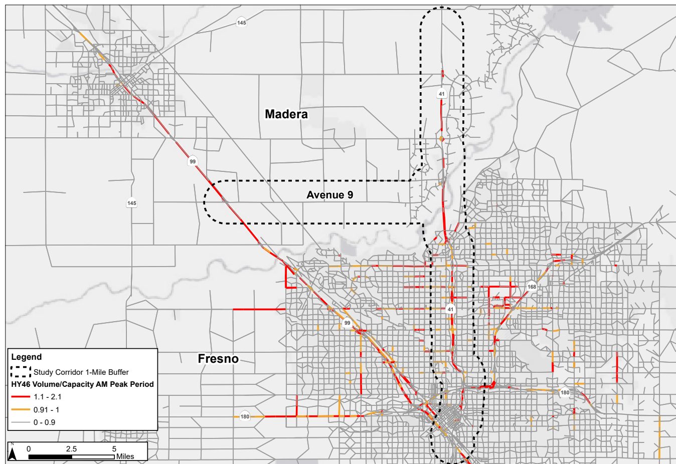
Figure 2.12: 2046 Horizon Year: Volume to Capacity AM Peak Period
